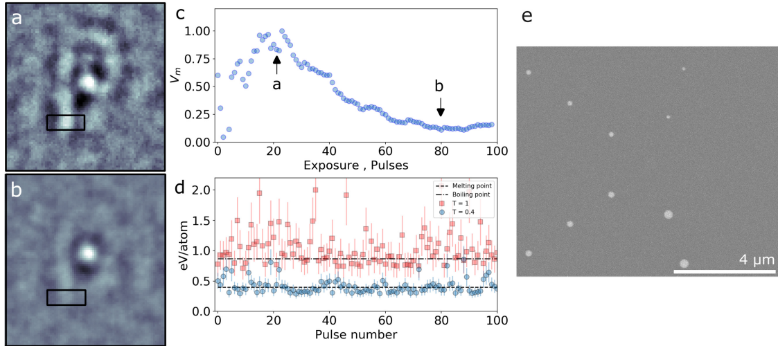
Figure 4. Reconstruction (real part of the image) obtained with a transmission T = 0.4 and exposure of a) 20 FEL pulses and b) 80 FEL pulses. c) Normalized variance obtained from the ROIs as a function of total accumulated pulse energy. The ROIs are denoted by the black rectangles in a) and b). The variance of a) and b) is depicted with the black arrows. d) Calculated maximum energy per Au atom in the sample as a function of pulse number. e) SEM image of the sample taken after the FEL study.
