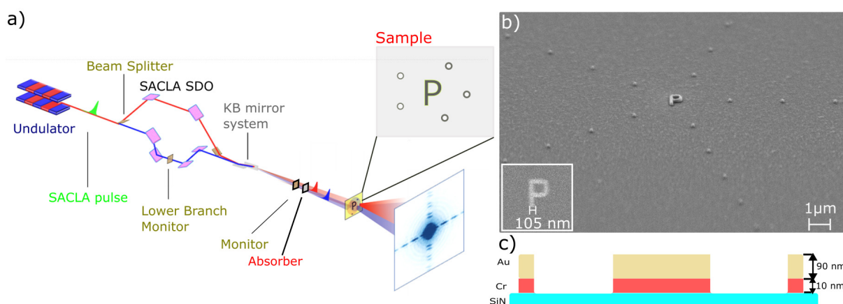
Figure 1. (a) Schematics of the hard X-ray FTH experiments using the SACLA SDO system. Each SASE pulse is split into two pulses using the SDO. The pulses are focused with the KB optics and travel in the sample direction with a delay time. Two beams illuminate the sample with a partial overlap. Holograms are collected by the detector. Time delay between the pulse pairs is defined by the SDO system. (b) SEM image of the selected sample (object and reference structures i.e., dots) on the silicon nitride membrane. The inset shows the zoom into the sample object (i.e., letter P). (c) Detailed cross-section of each sample structure.
