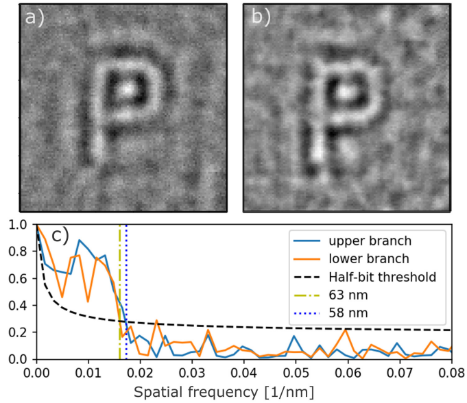
Figure 3. Reconstruction (real part of the image) obtained with the a) upper and b) lower branch of SDO system, respectively. c) FRC analysis of the reconstructions shown in a) and b). Black dashed line corresponds to half-bit threshold 33 . Vertical blue and yellow lines denote the resolution of the reconstructions of 58 nm and 63 nm for the upper and lower branch, respectively.
